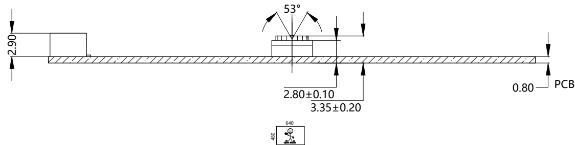
SIDE VIEW
